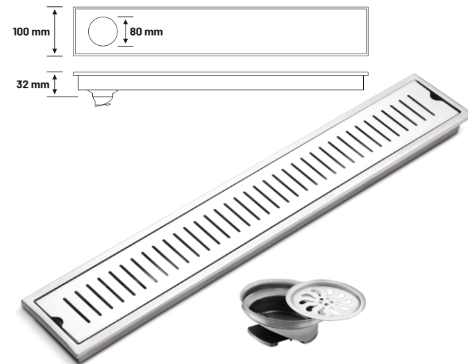
Channel Drain - CCD03
