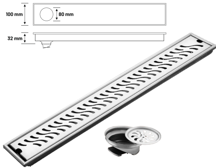
Channel Drain - CCD01
