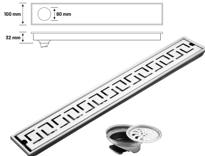
Channel Drain - CCD04
