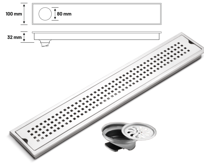
Channel Drain - CCD02
