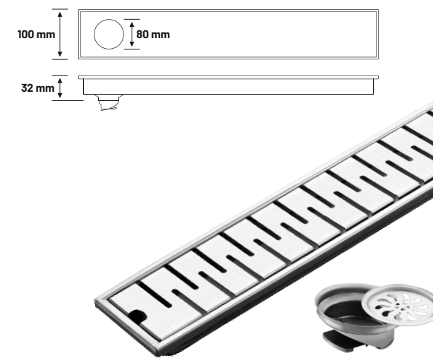
Channel Drain - CCD05
